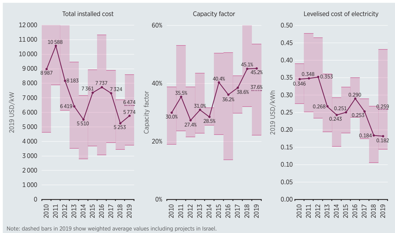
Figure 1.7 Global weighted average total installed costs, capacity factors and LCOE for CSP, 2010-2019
